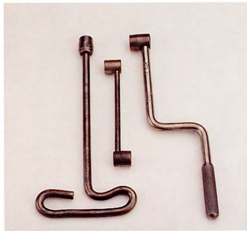
The three 1920s pieces pictured here have non-detachable ends. They have the Snap-on logo, no year mark, one alphabet and 2 numbers. They may have been a part of an automotive set. No price available.
